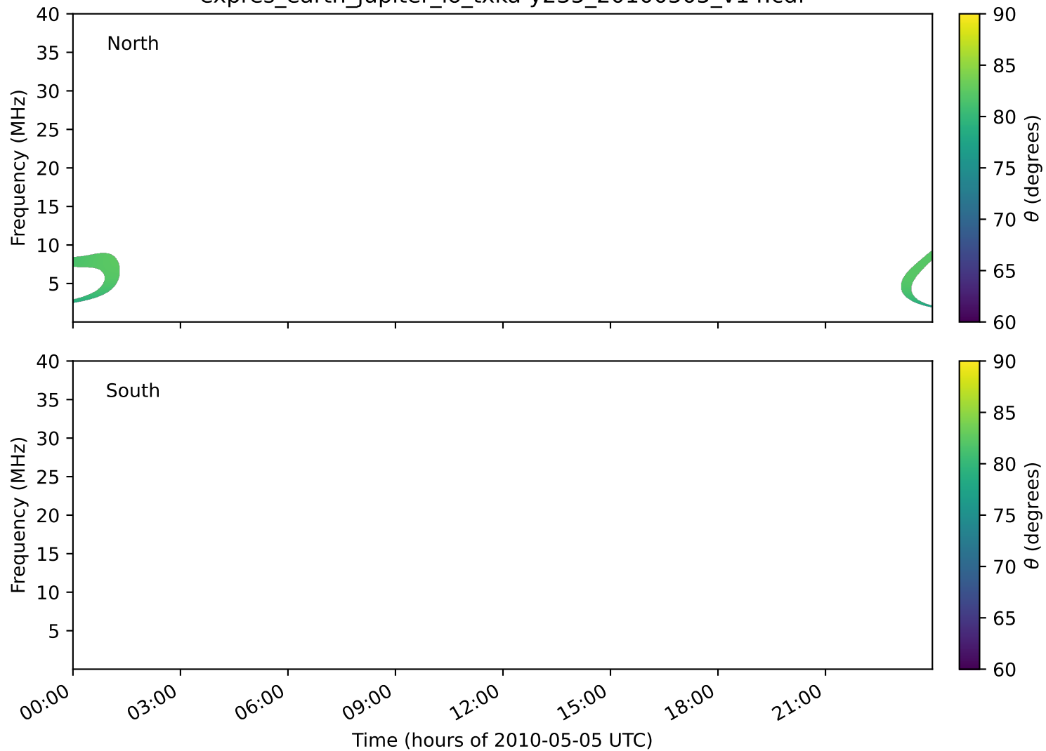
expres_earth_jupiter_io_txka-y235_20100505_v14.cdf
