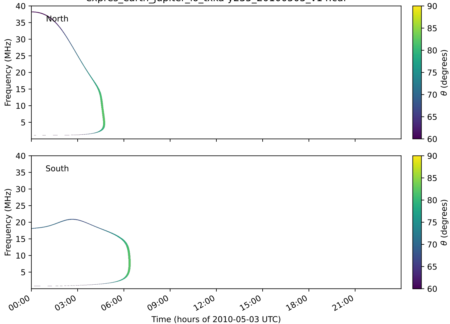
expres_earth_jupiter_io_txka-y235_20100503_v14.cdf
