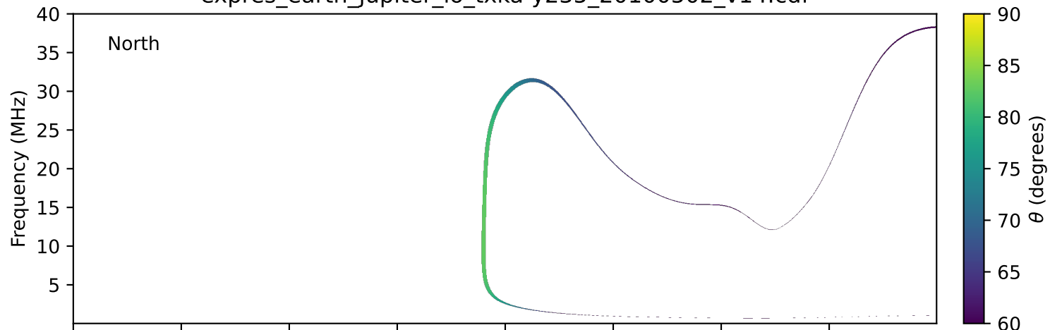
expres_earth_jupiter_io_txka-y235_20100502_v14.cdf
