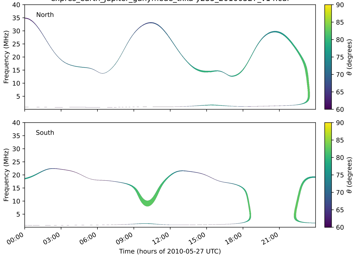
expres_earth_jupiter_ganymede_txka-y235_20100527_v14.cdf
