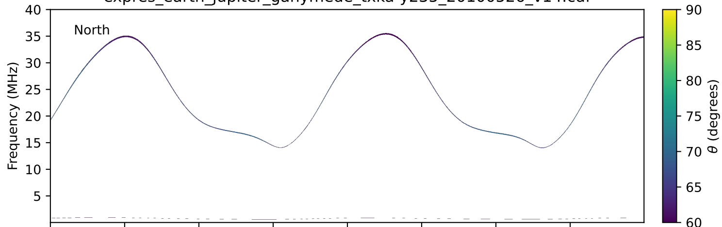
expres_earth_jupiter_ganymede_txka-y235_20100526_v14.cdf
