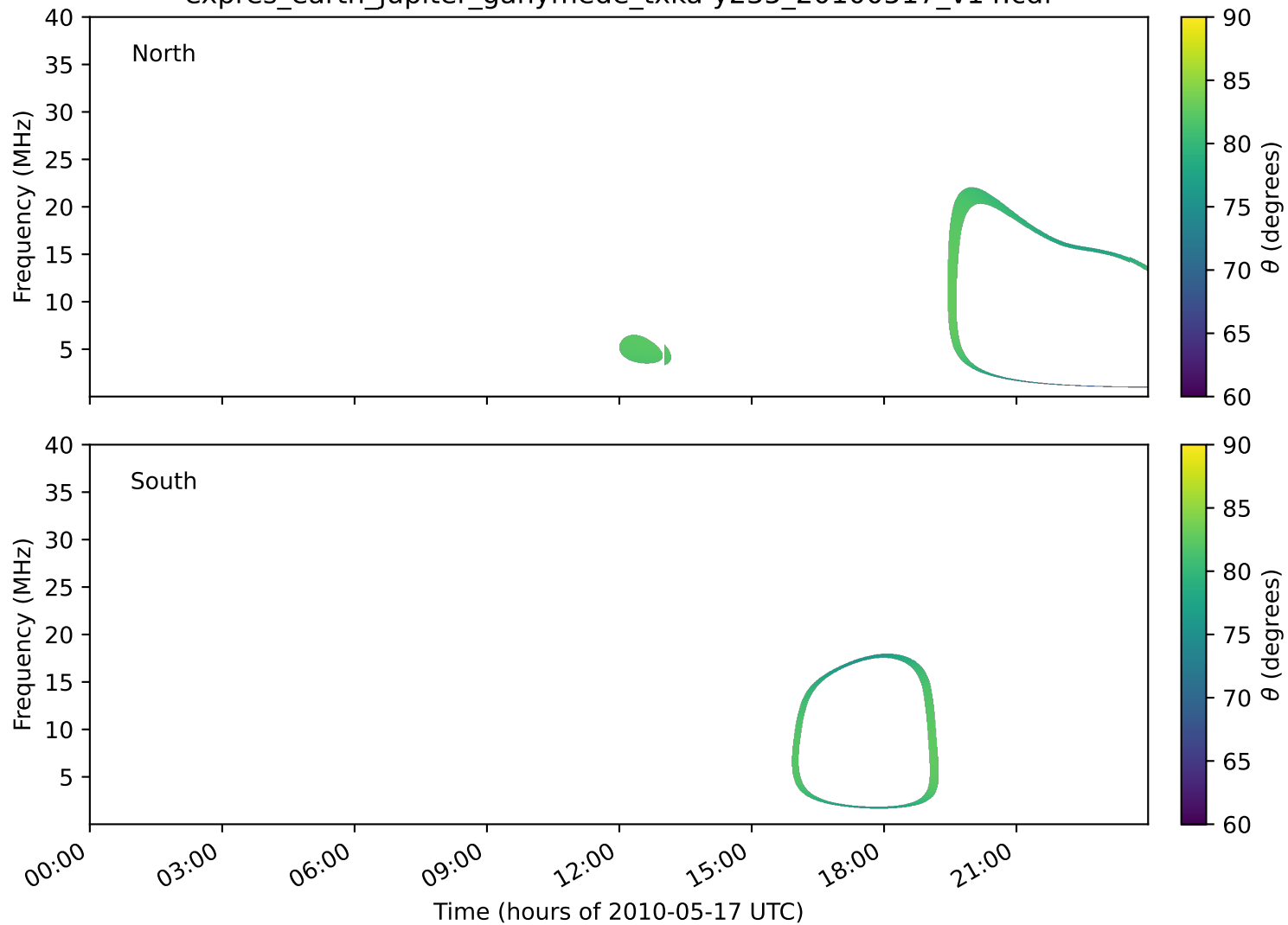
expres_earth_jupiter_ganymede_txka-y235_20100517_v14.cdf
