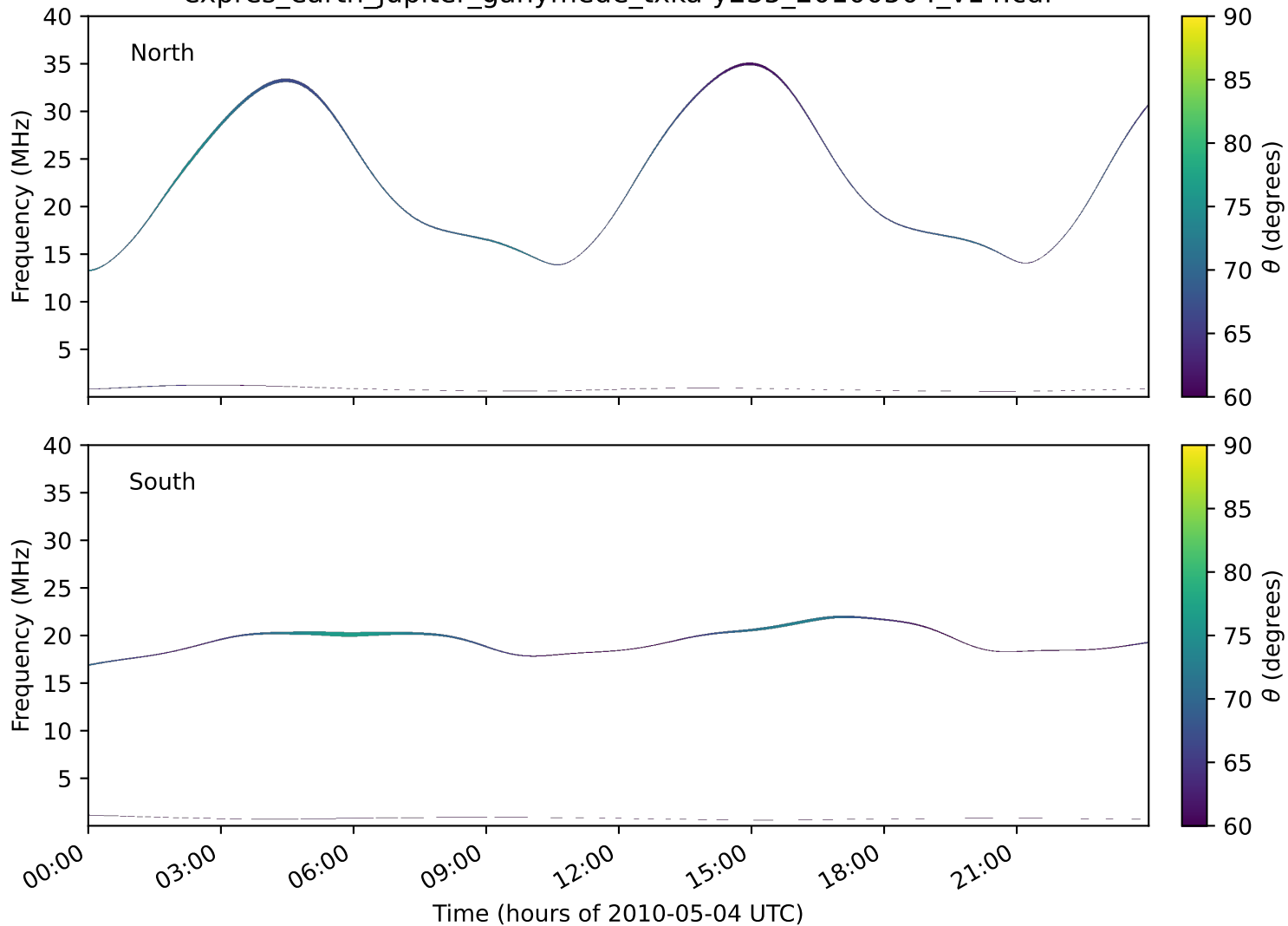
expres_earth_jupiter_ganymede_txka-y235_20100504_v14.cdf
