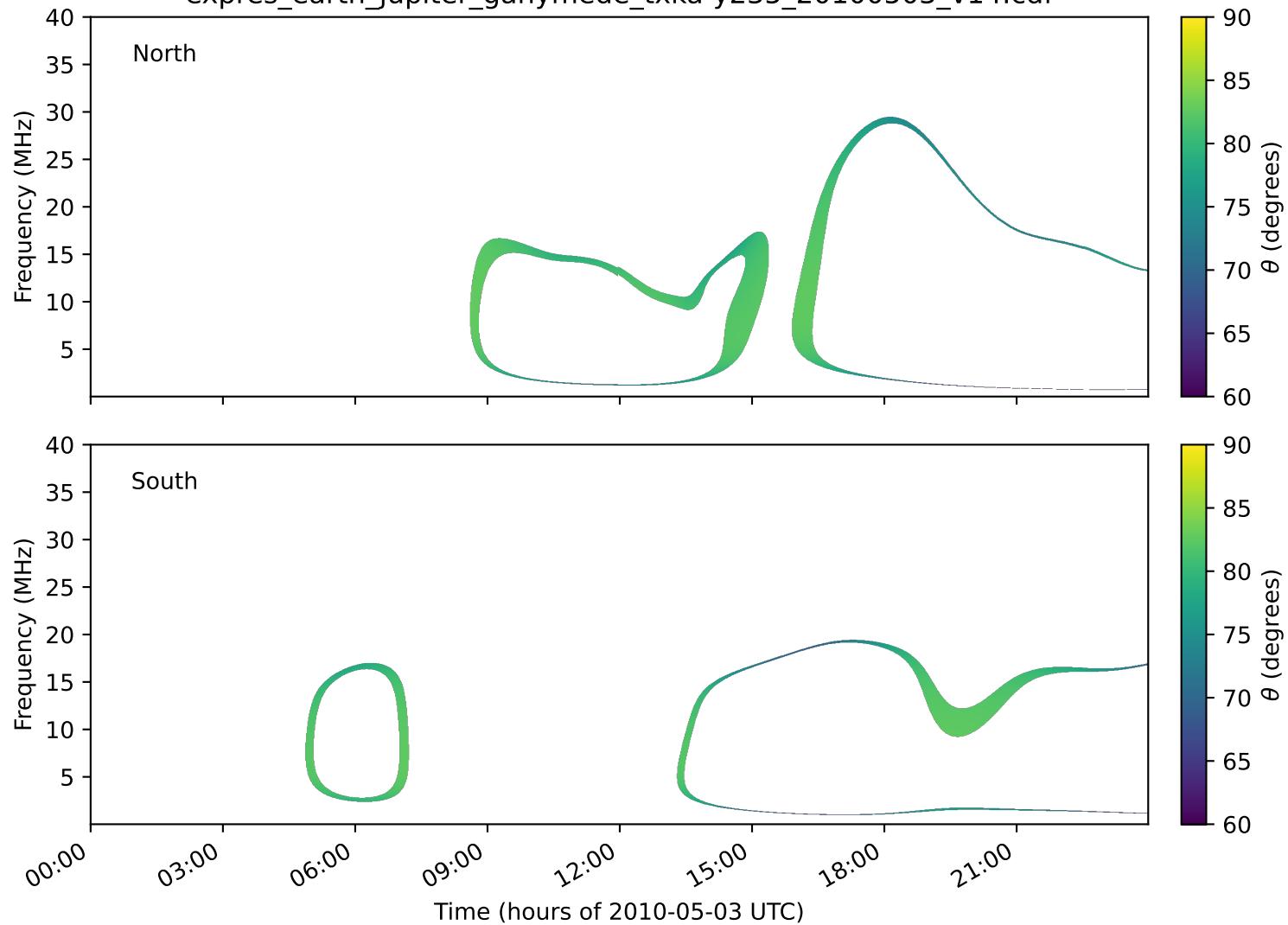
expres_earth_jupiter_ganymede_txka-y235_20100503_v14.cdf
