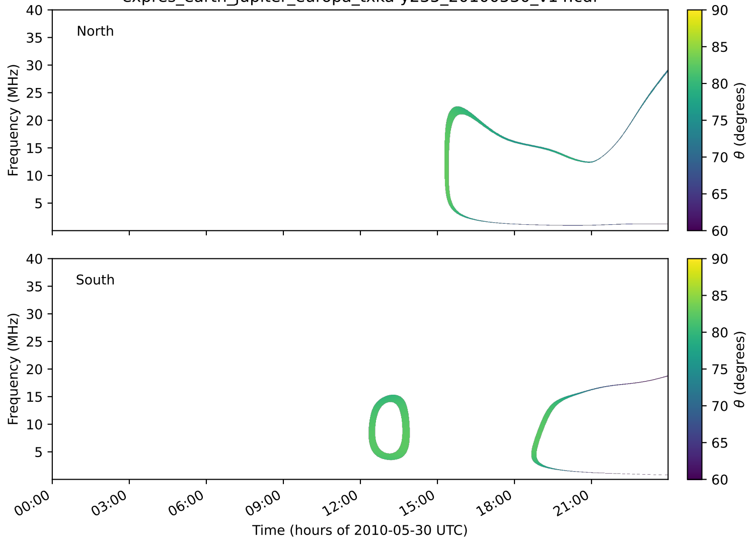
expres_earth_jupiter_europa_txka-y235_20100530_v14.cdf
