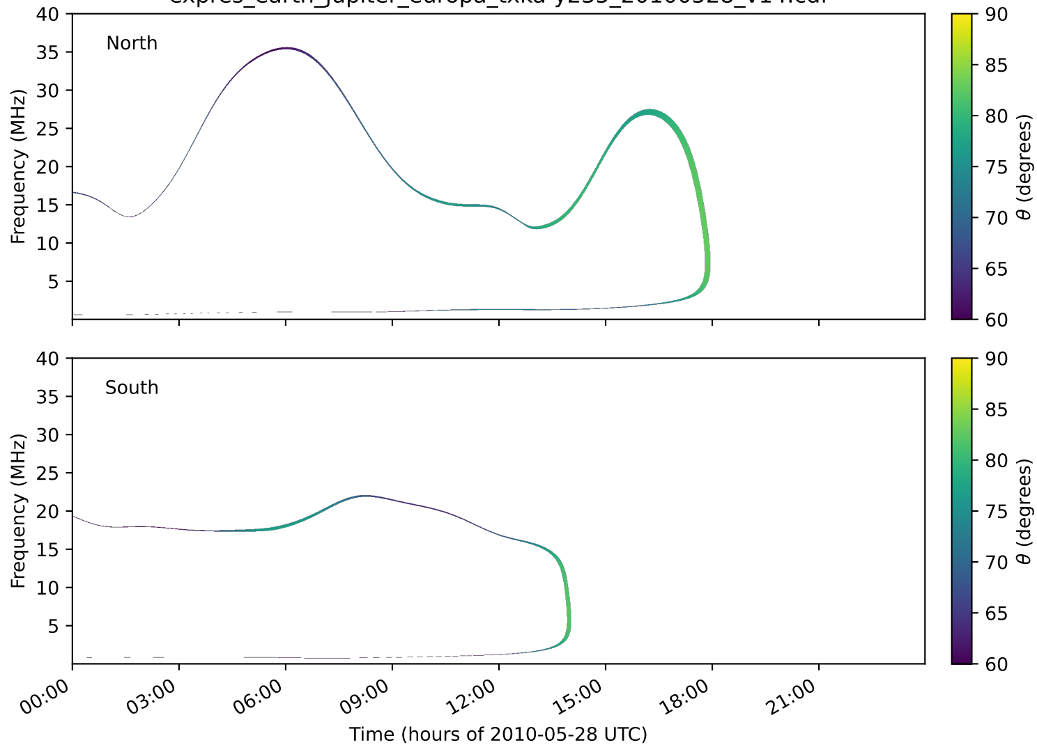
expres_earth_jupiter_europa_txka-y235_20100528_v14.cdf
