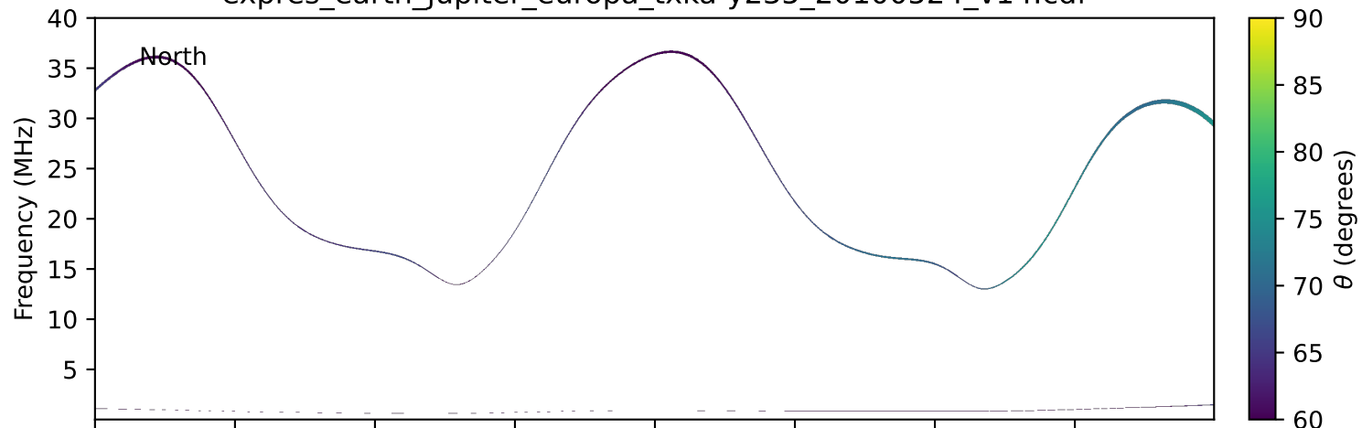
expres_earth_jupiter_europa_txka-y235_20100524_v14.cdf
