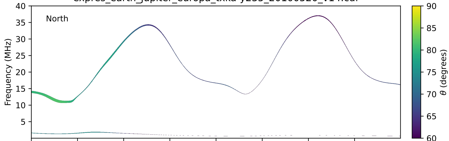
expres_earth_jupiter_europa_txka-y235_20100520_v14.cdf
