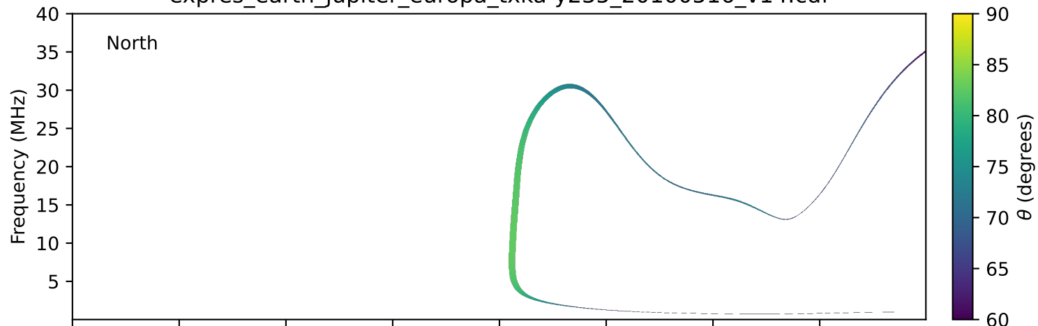
expres_earth_jupiter_europa_txka-y235_20100516_v14.cdf
