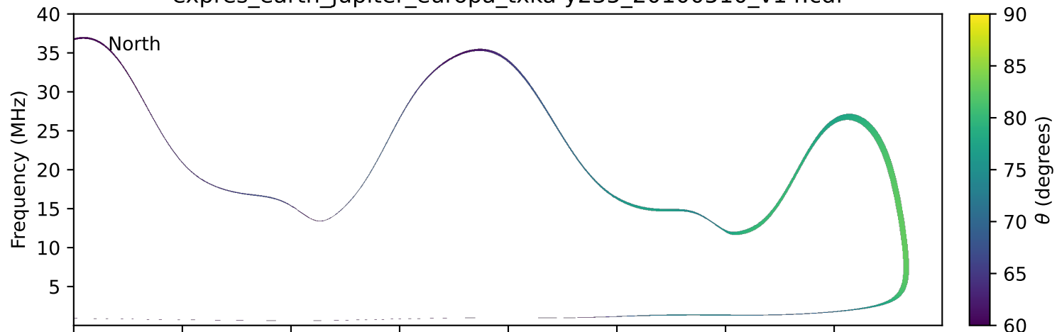
expres_earth_jupiter_europa_txka-y235_20100510_v14.cdf
