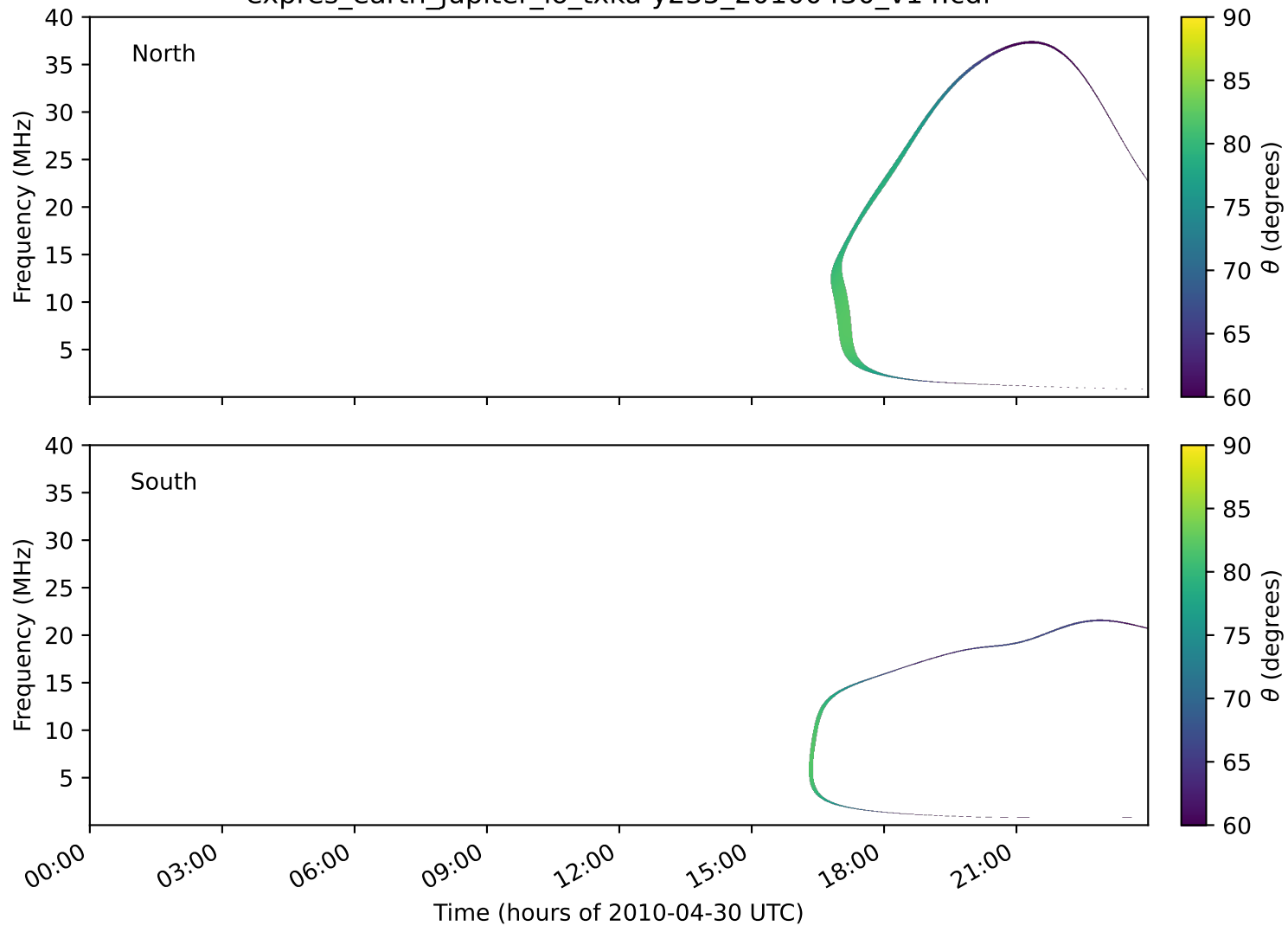
expres_earth_jupiter_io_txka-y235_20100430_v14.cdf
