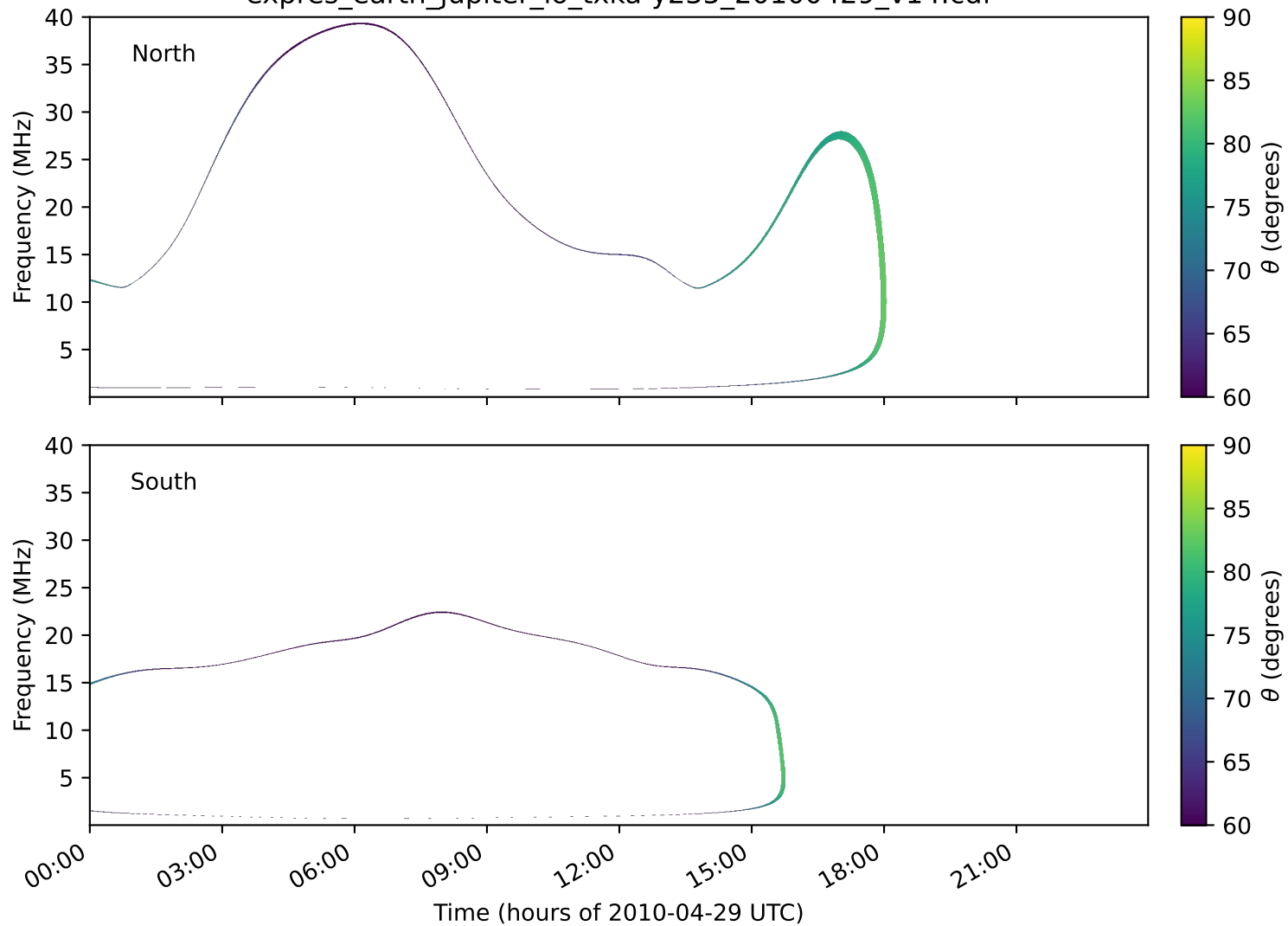
expres_earth_jupiter_io_txka-y235_20100429_v14.cdf
