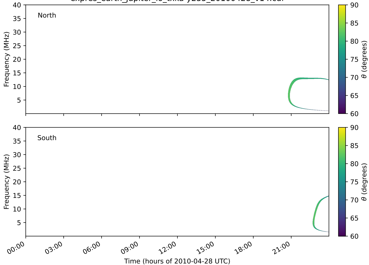
expres_earth_jupiter_io_txka-y235_20100428_v14.cdf
