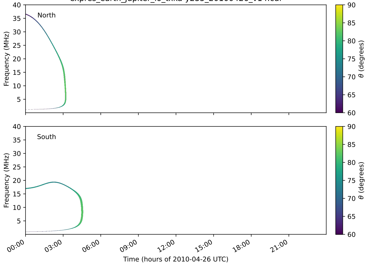
expres_earth_jupiter_io_txka-y235_20100426_v14.cdf
