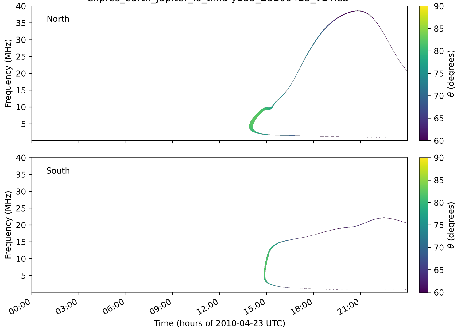
expres_earth_jupiter_io_txka-y235_20100423_v14.cdf
