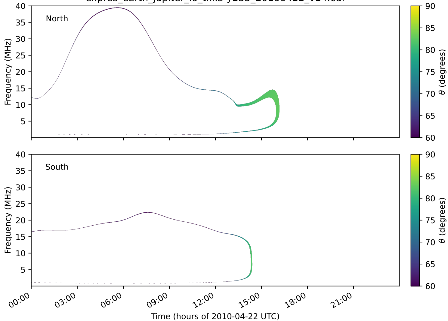
expres_earth_jupiter_io_txka-y235_20100422_v14.cdf
