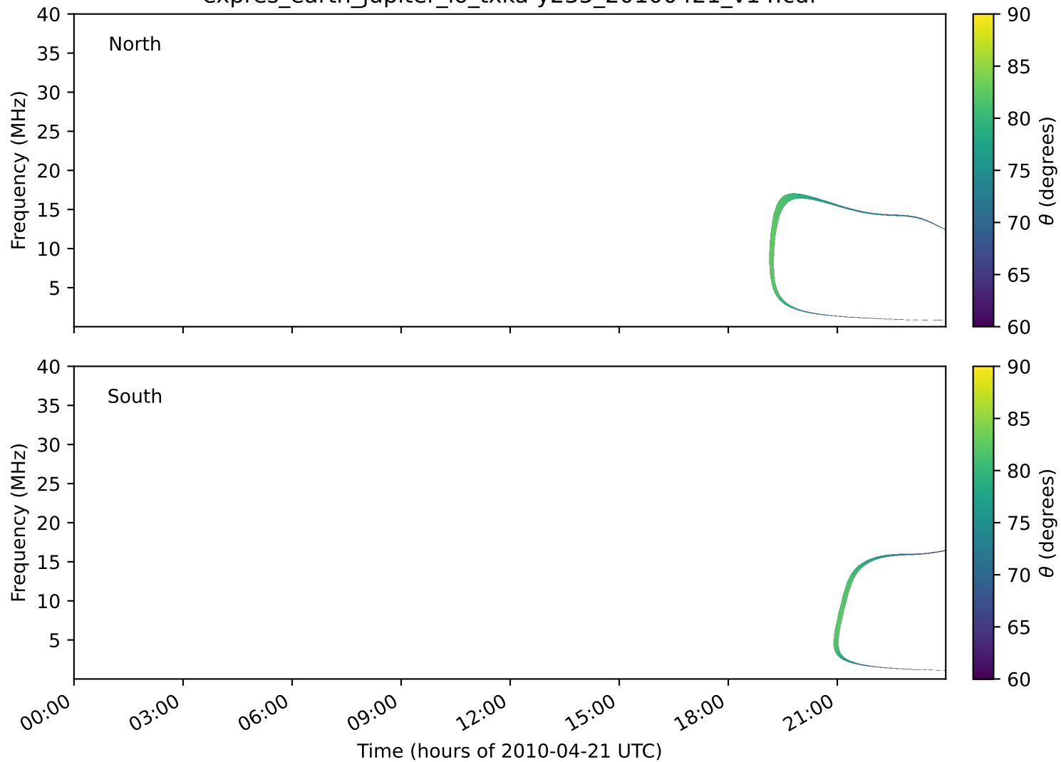
expres_earth_jupiter_io_txka-y235_20100421_v14.cdf
