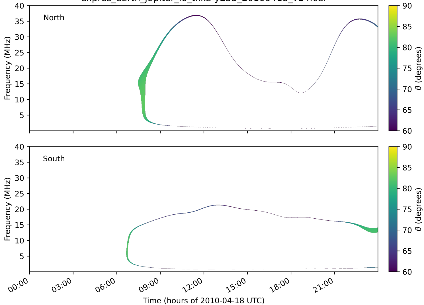
expres_earth_jupiter_io_txka-y235_20100418_v14.cdf
