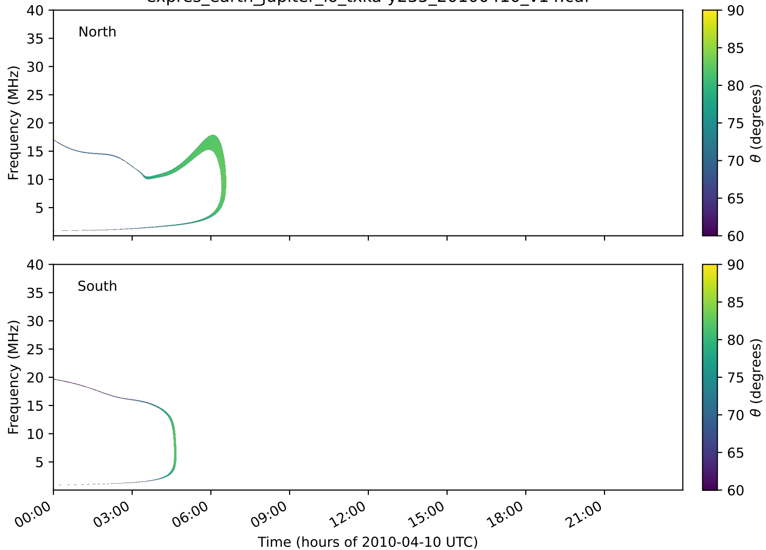
expres_earth_jupiter_io_txka-y235_20100410_v14.cdf
