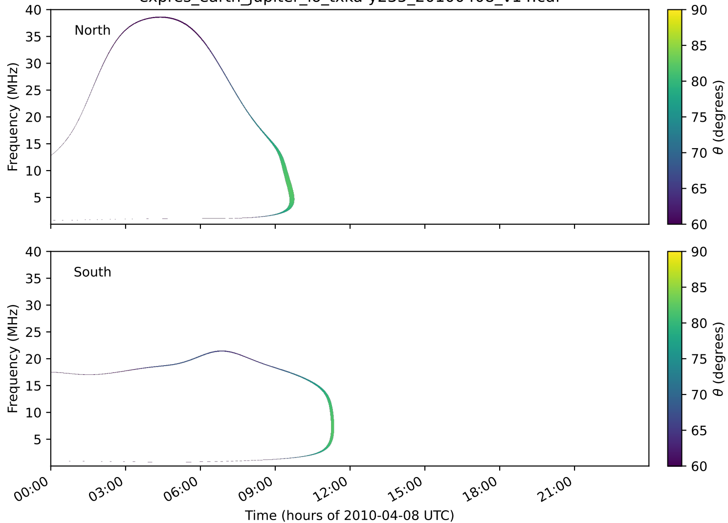
expres_earth_jupiter_io_txka-y235_20100408_v14.cdf
