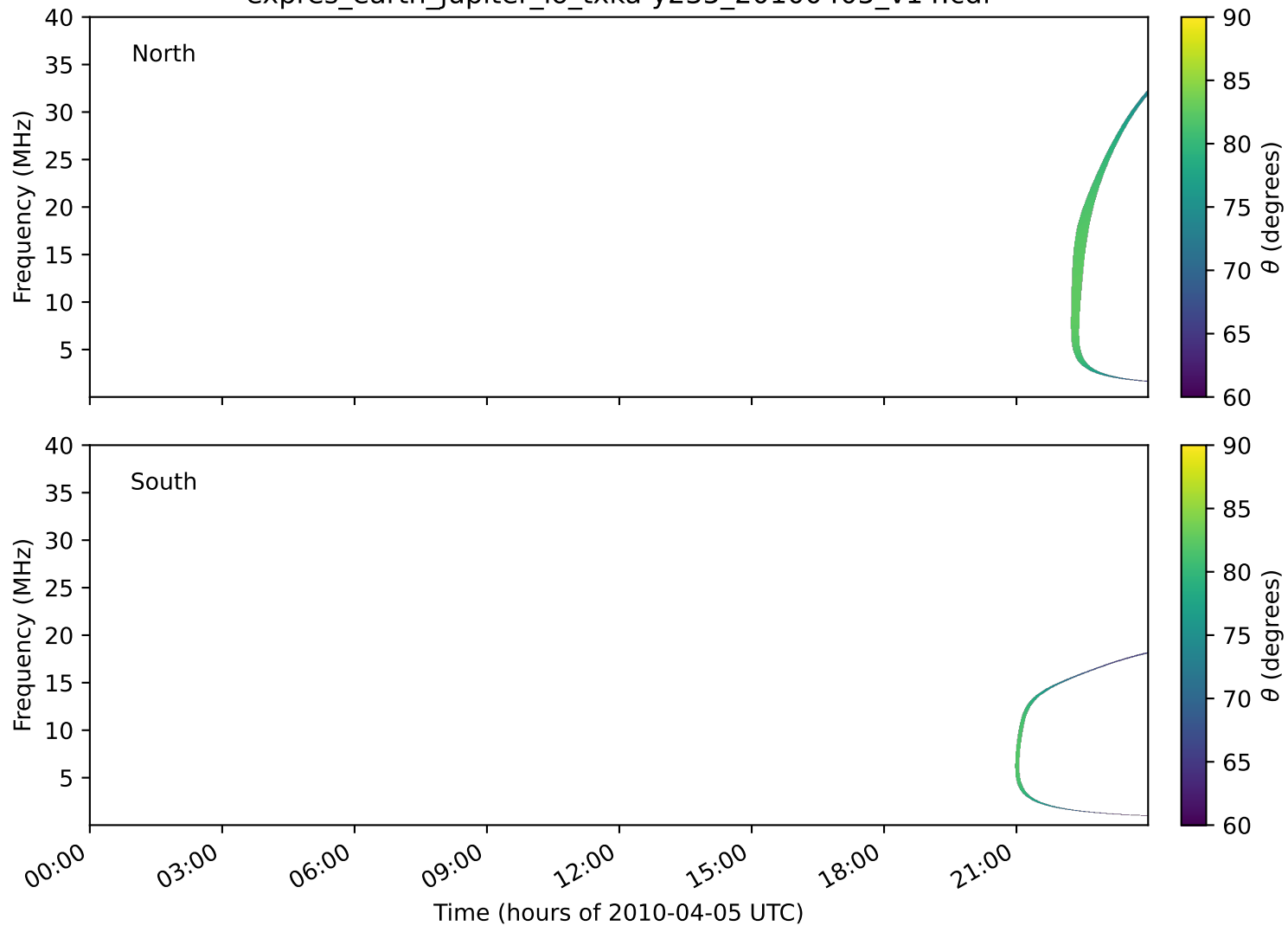
expres_earth_jupiter_io_txka-y235_20100405_v14.cdf
