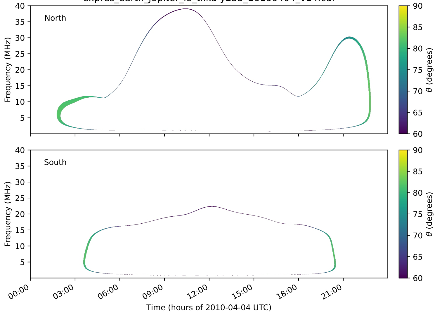
expres_earth_jupiter_io_txka-y235_20100404_v14.cdf
