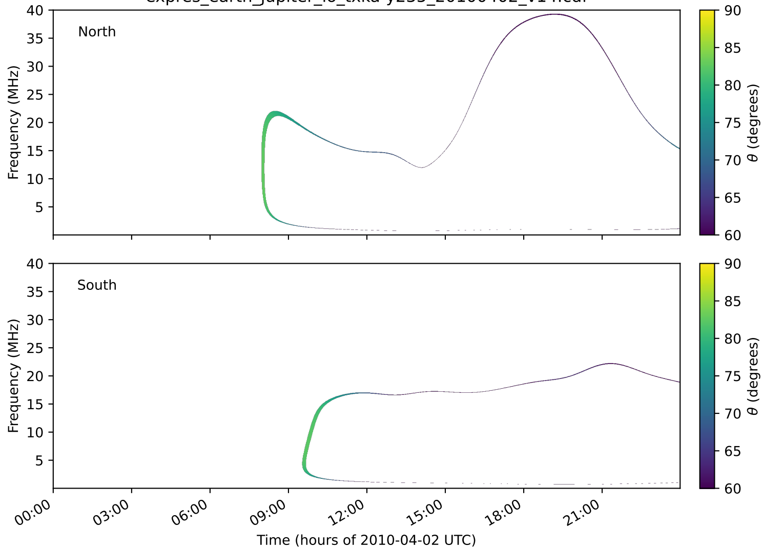
expres_earth_jupiter_io_txka-y235_20100402_v14.cdf
