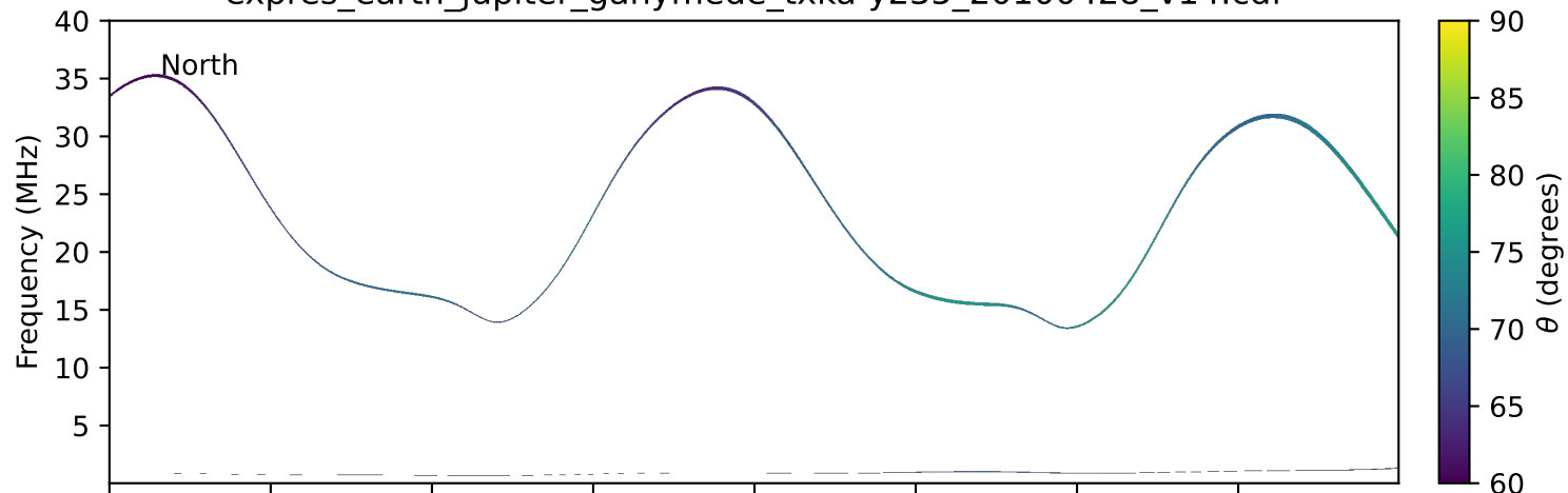
expres_earth_jupiter_ganymede_txka-y235_20100428_v14.cdf
