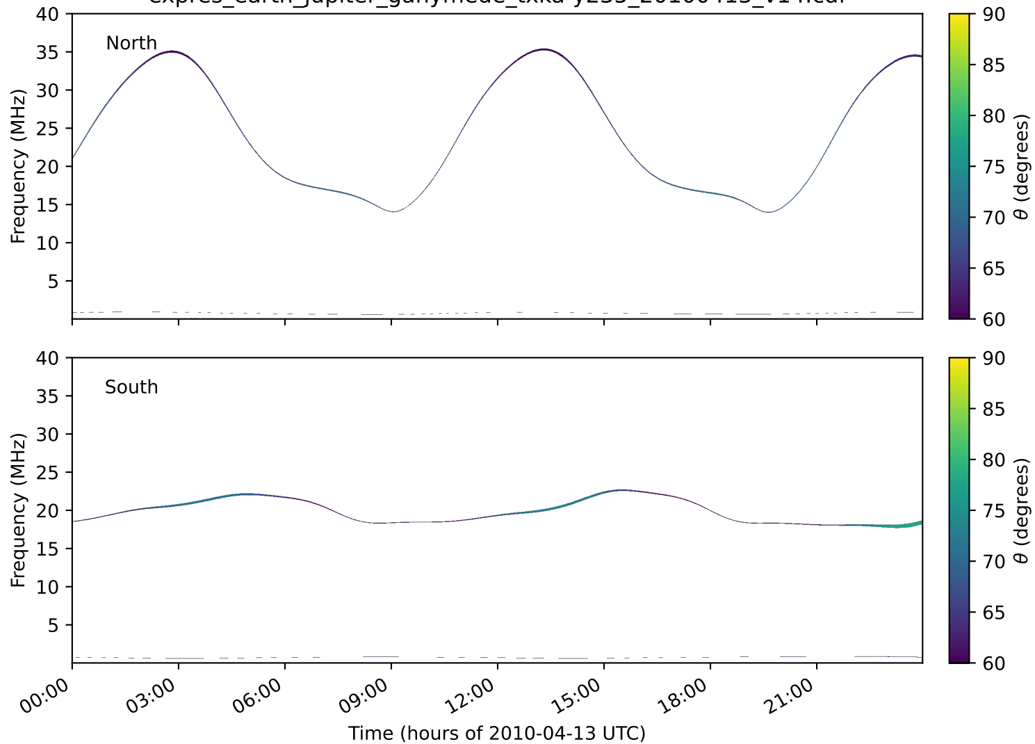
expres_earth_jupiter_ganymede_txka-y235_20100413_v14.cdf
