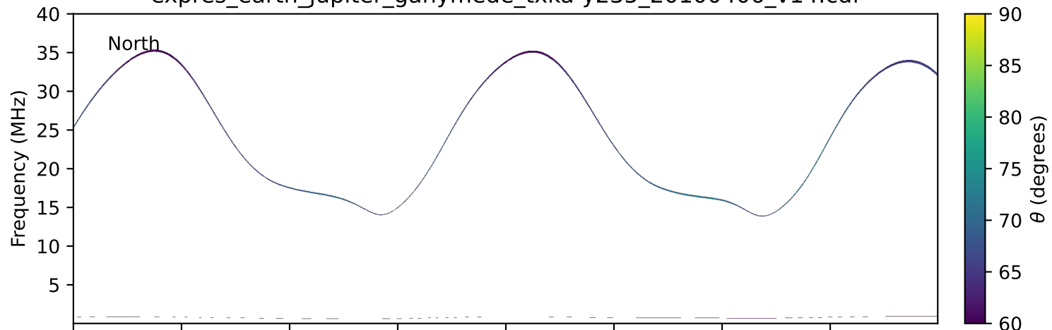
expres_earth_jupiter_ganymede_txka-y235_20100406_v14.cdf
