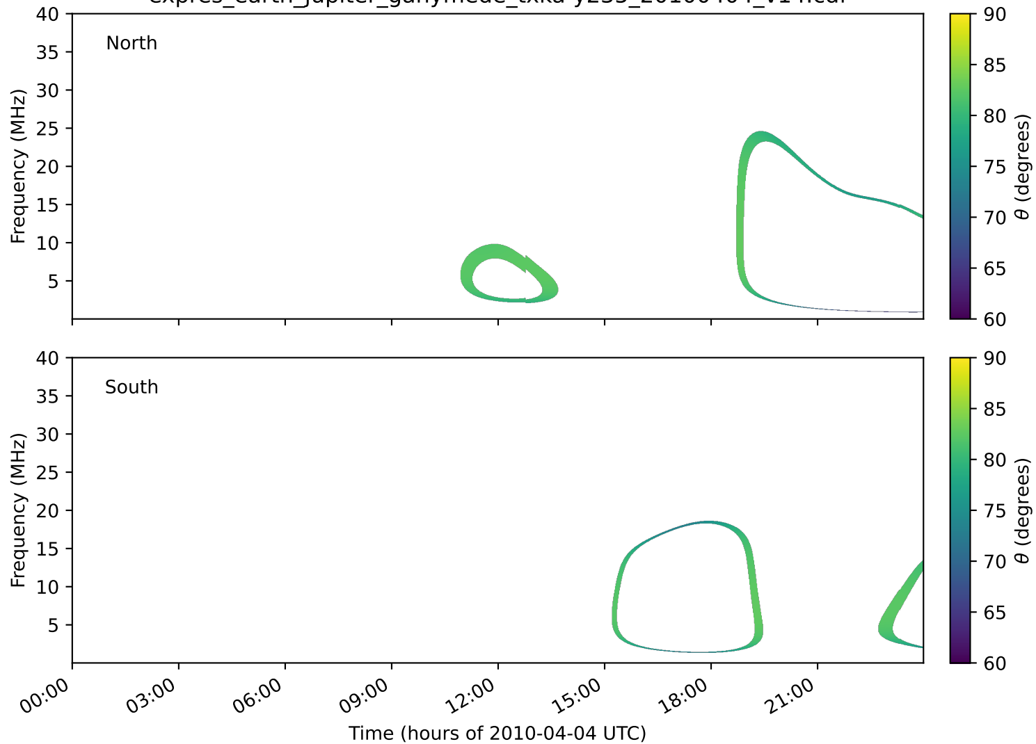
expres_earth_jupiter_ganymede_txka-y235_20100404_v14.cdf
