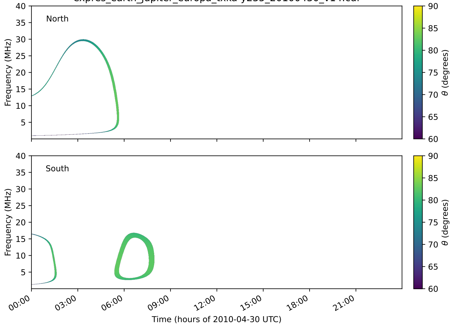
expres_earth_jupiter_europa_txka-y235_20100430_v14.cdf
