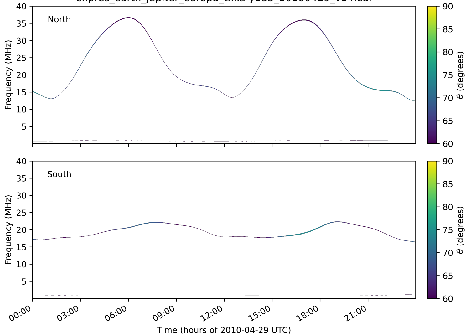
expres_earth_jupiter_europa_txka-y235_20100429_v14.cdf
