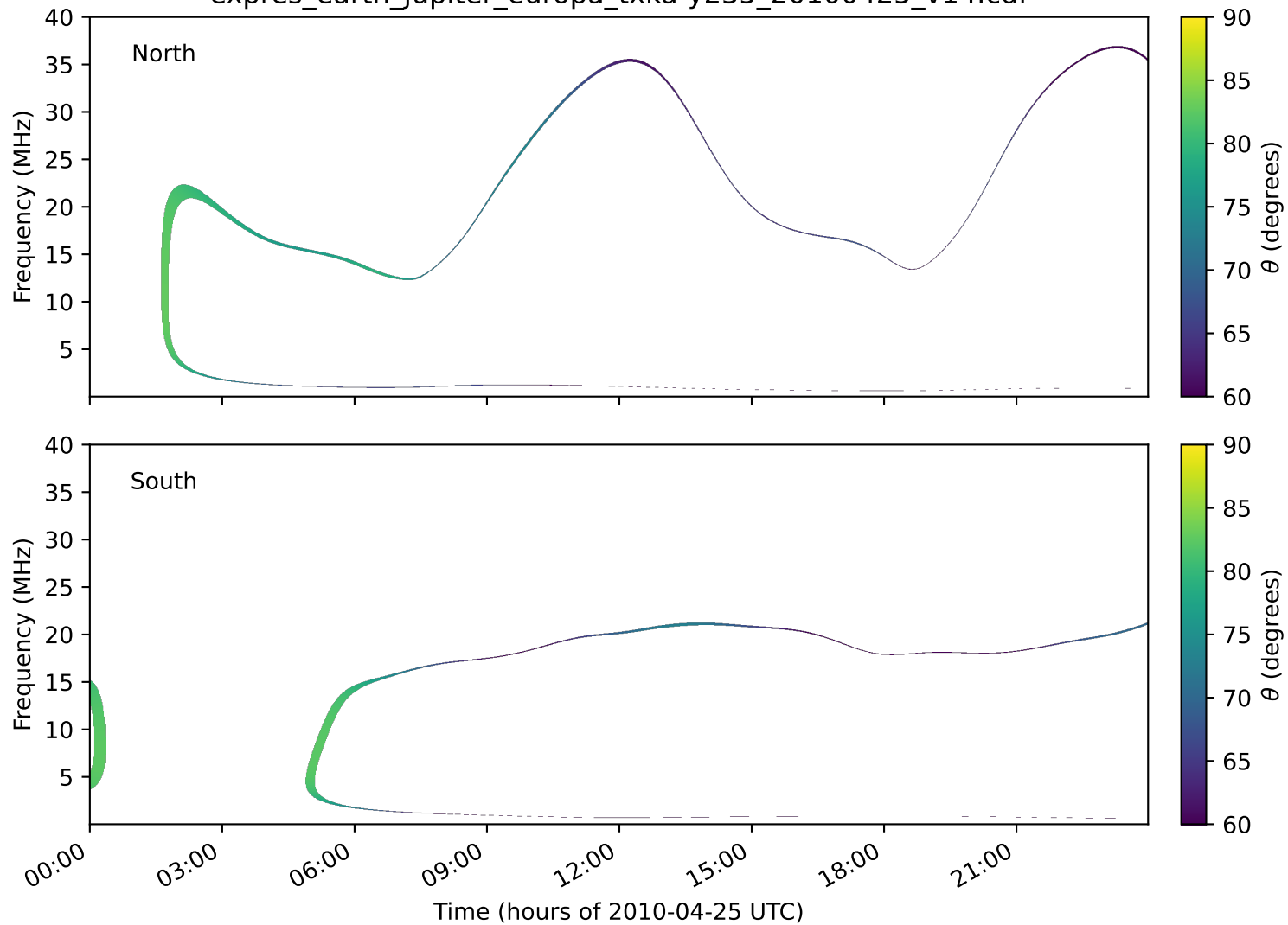
expres_earth_jupiter_europa_txka-y235_20100425_v14.cdf
