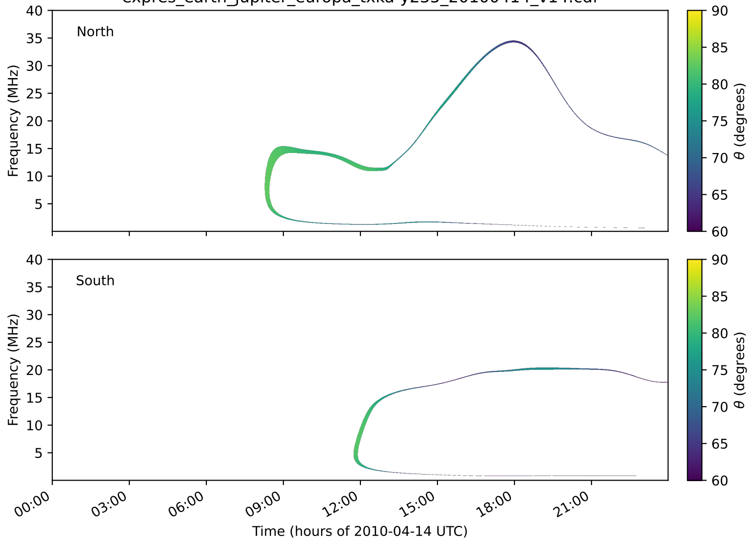
expres_earth_jupiter_europa_txka-y235_20100414_v14.cdf
