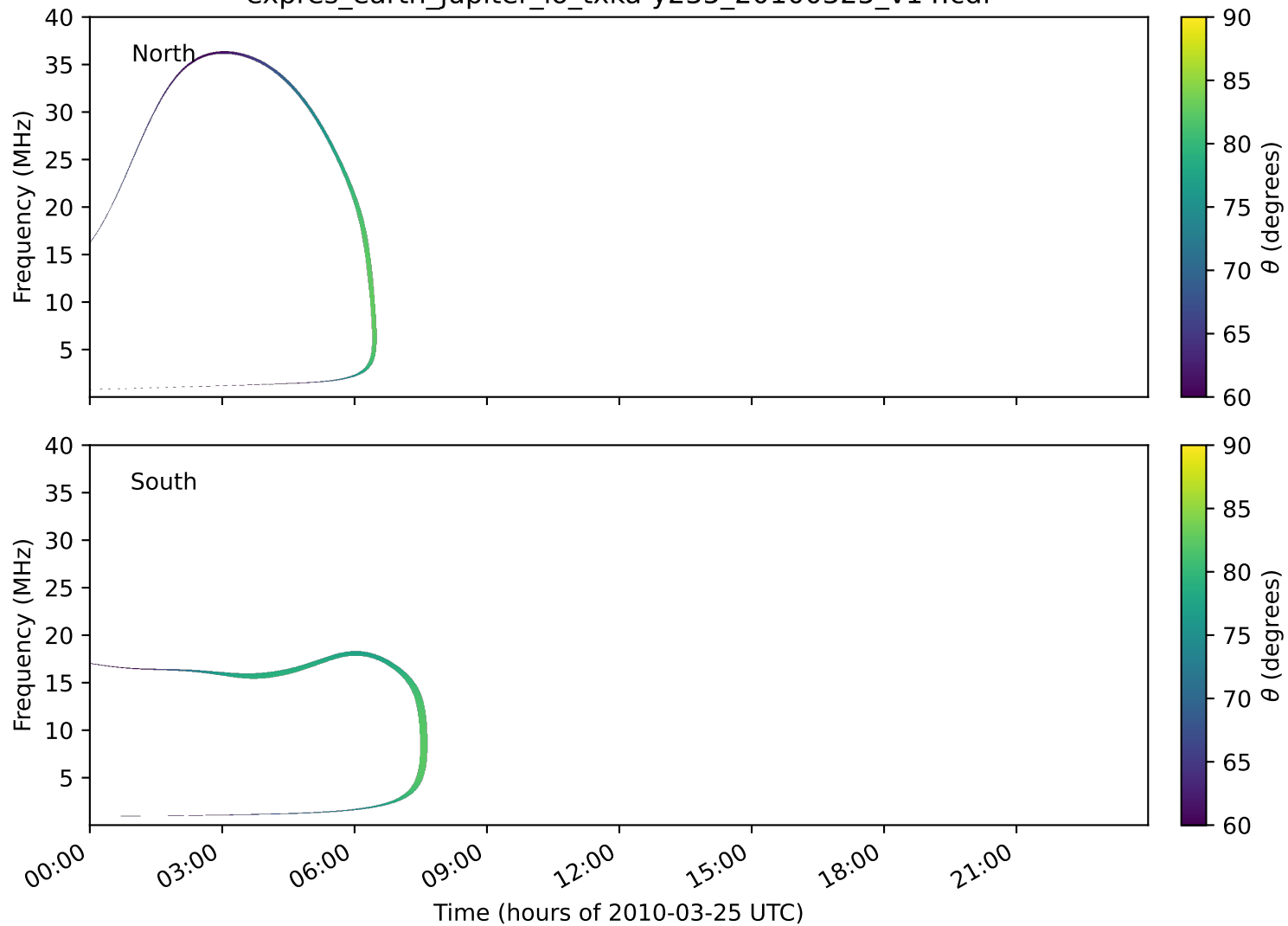
expres_earth_jupiter_io_txka-y235_20100325_v14.cdf
