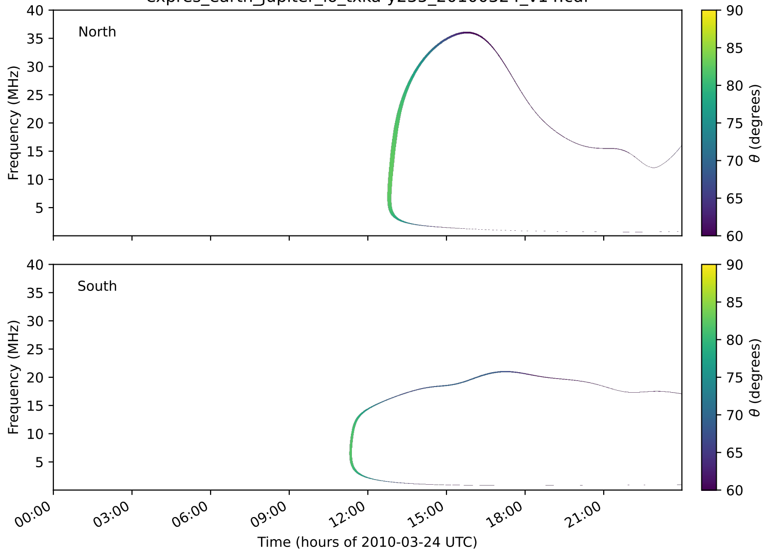
expres_earth_jupiter_io_txka-y235_20100324_v14.cdf
