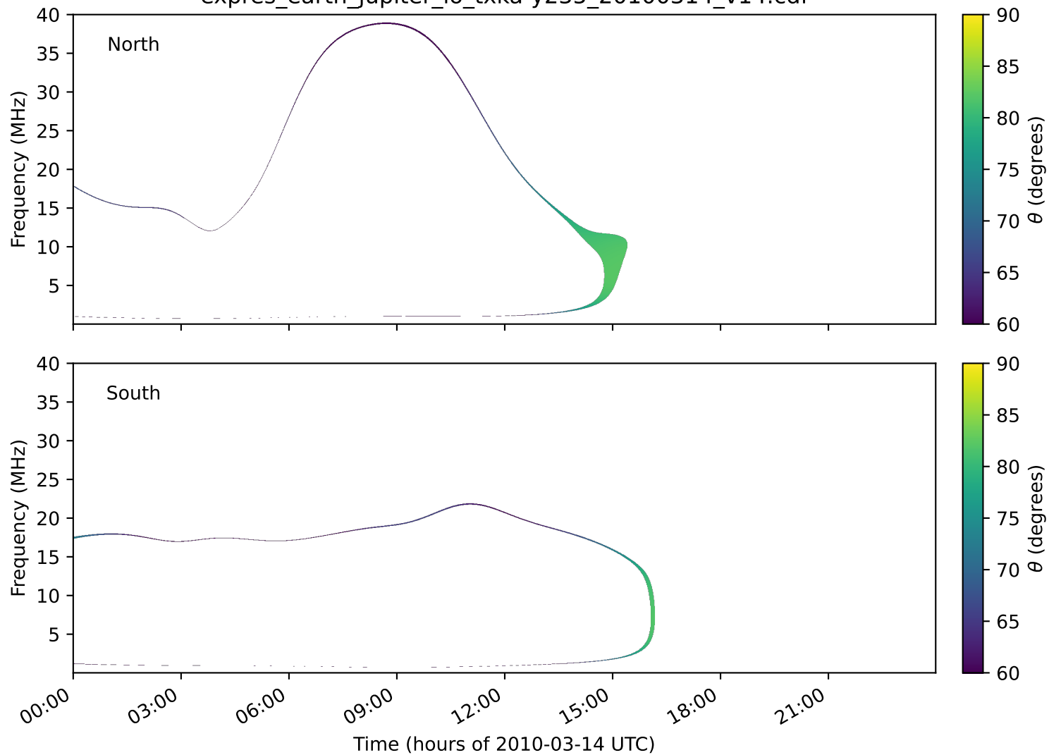
expres_earth_jupiter_io_txka-y235_20100314_v14.cdf
