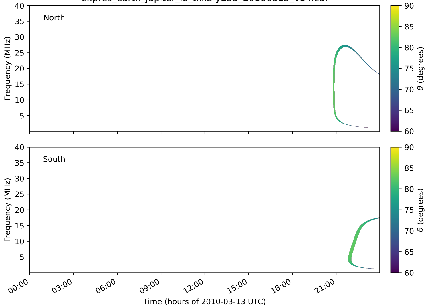
expres_earth_jupiter_io_txka-y235_20100313_v14.cdf
