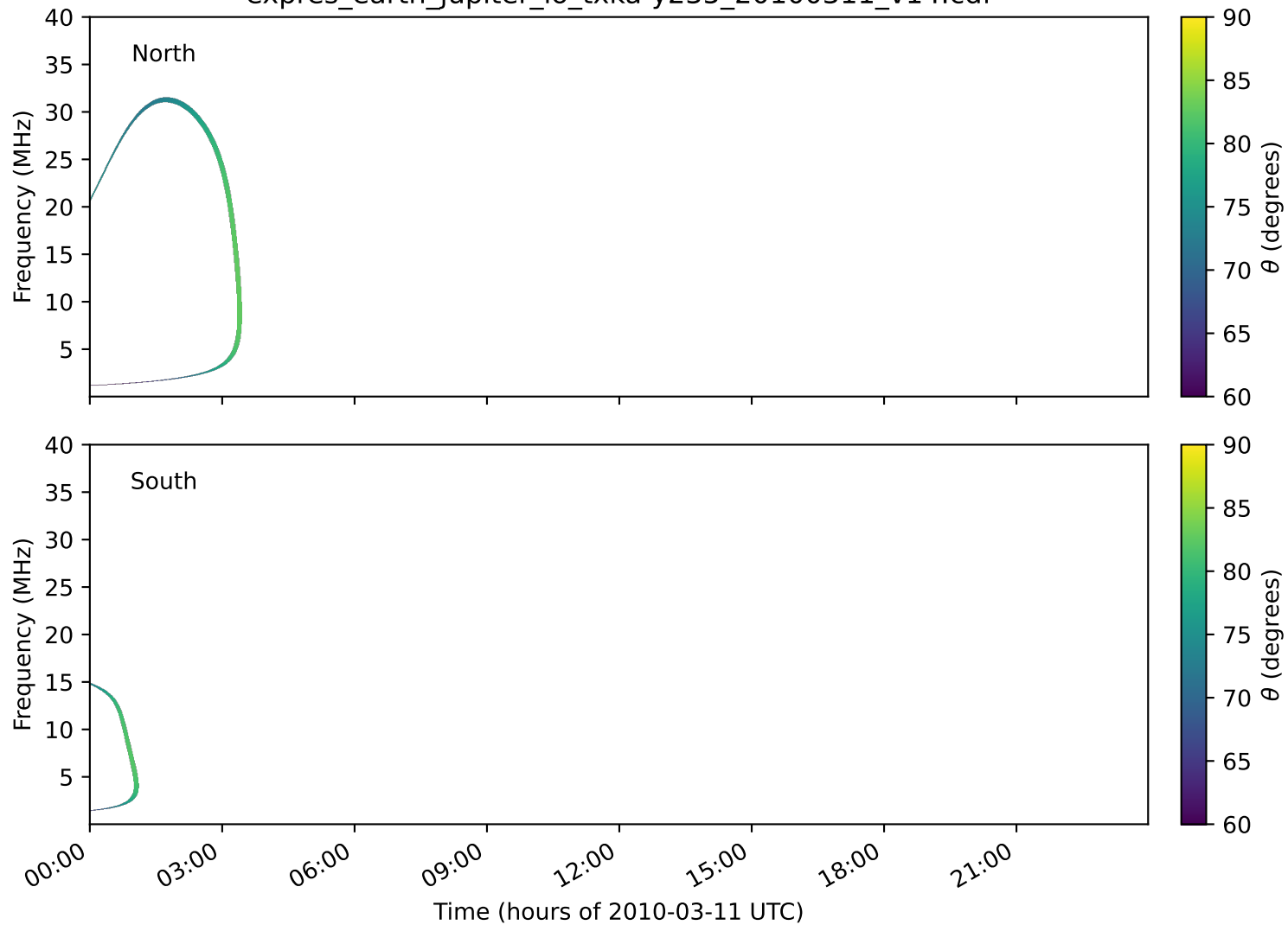
expres_earth_jupiter_io_txka-y235_20100311_v14.cdf
