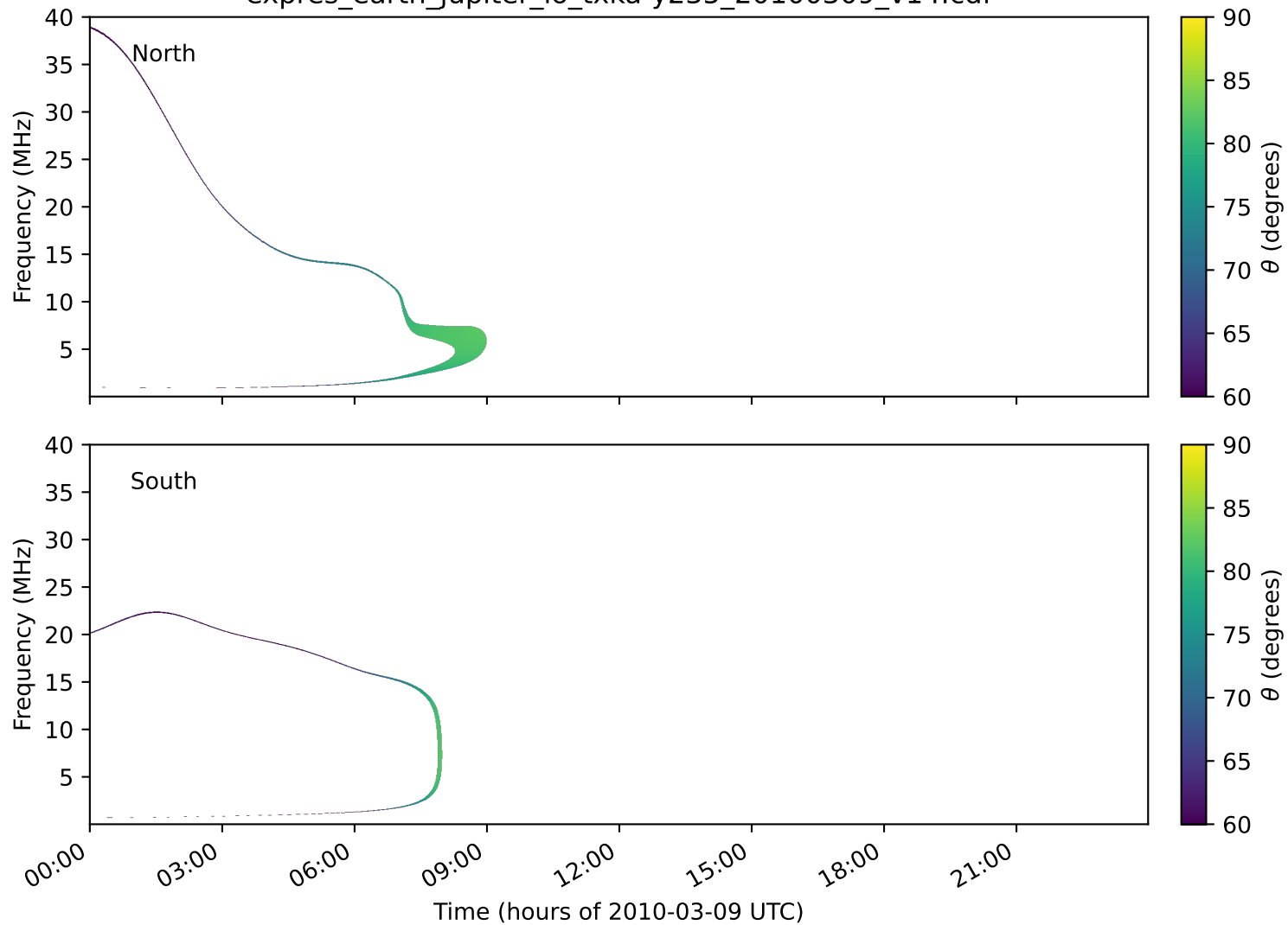
expres_earth_jupiter_io_txka-y235_20100309_v14.cdf
