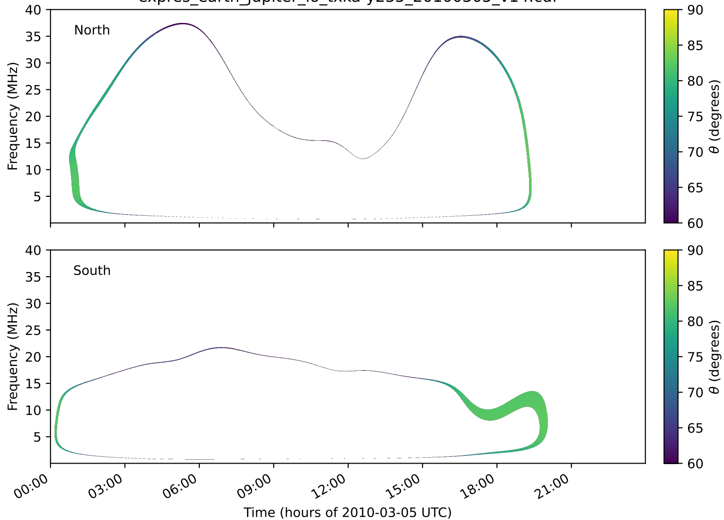
expres_earth_jupiter_io_txka-y235_20100305_v14.cdf
