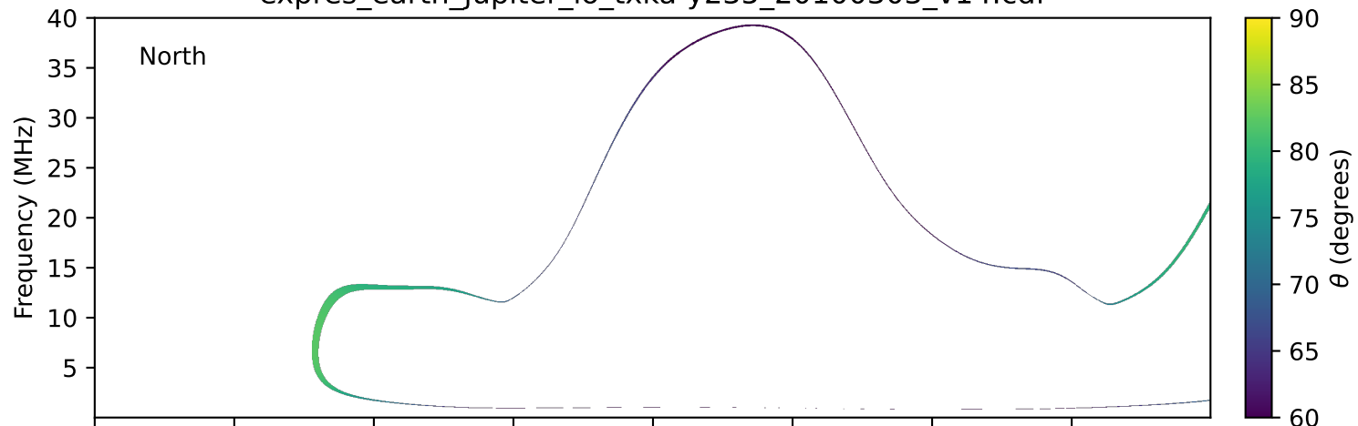
expres_earth_jupiter_io_txka-y235_20100303_v14.cdf
