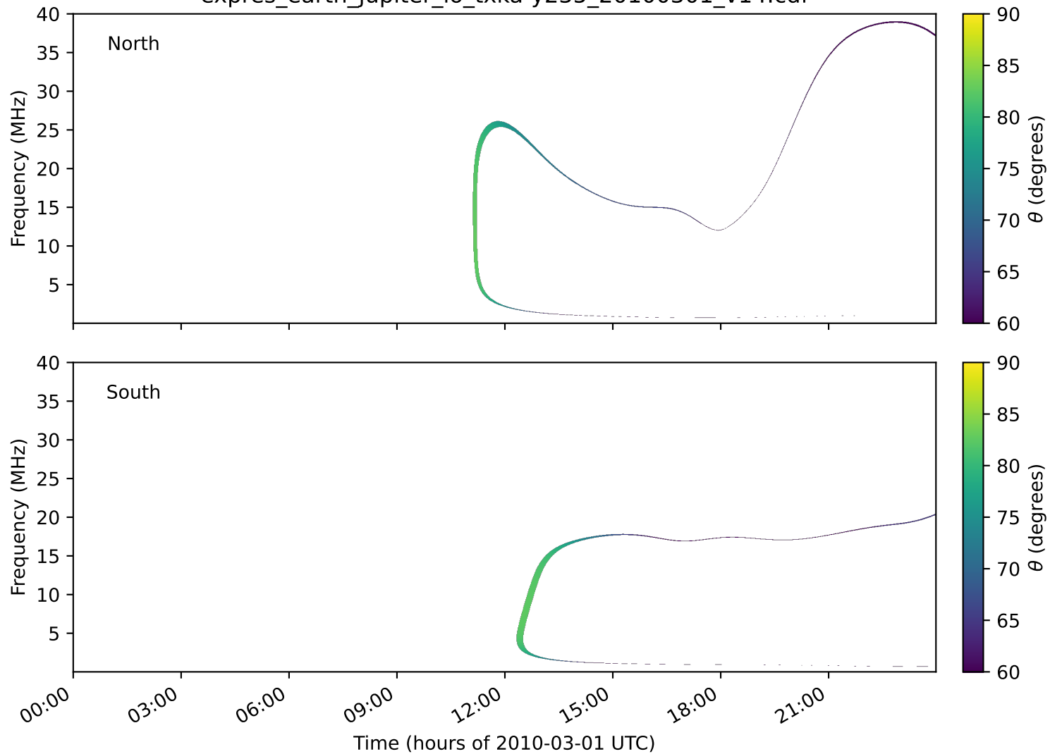
expres_earth_jupiter_io_txka-y235_20100301_v14.cdf
