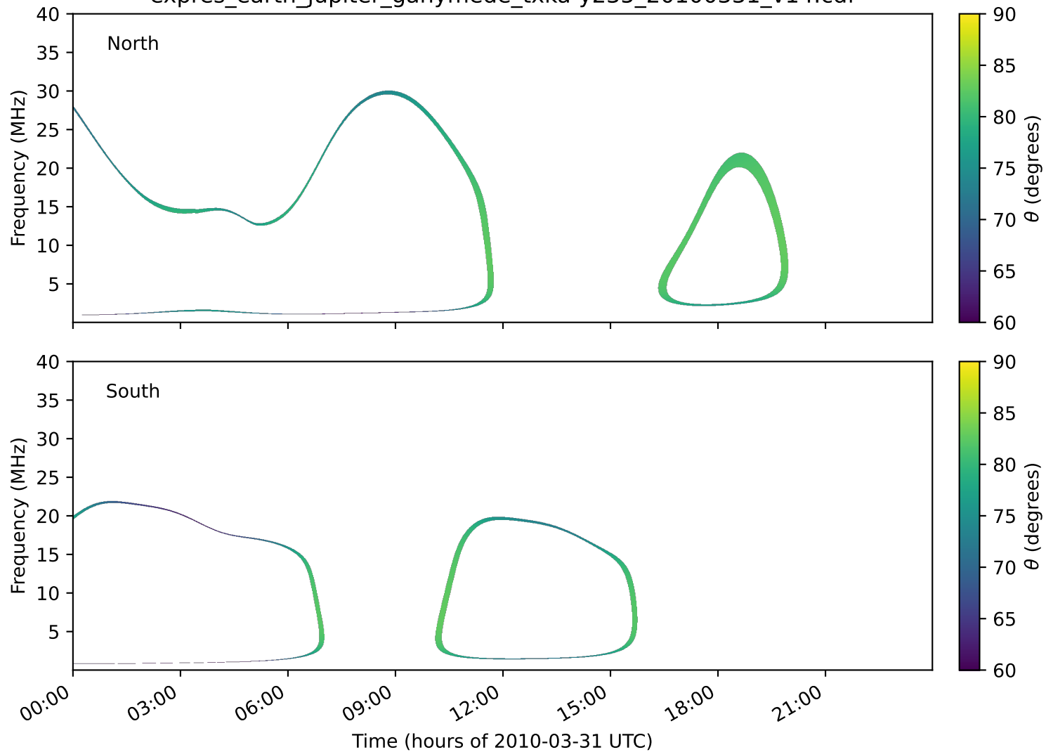
expres_earth_jupiter_ganymede_txka-y235_20100331_v14.cdf
