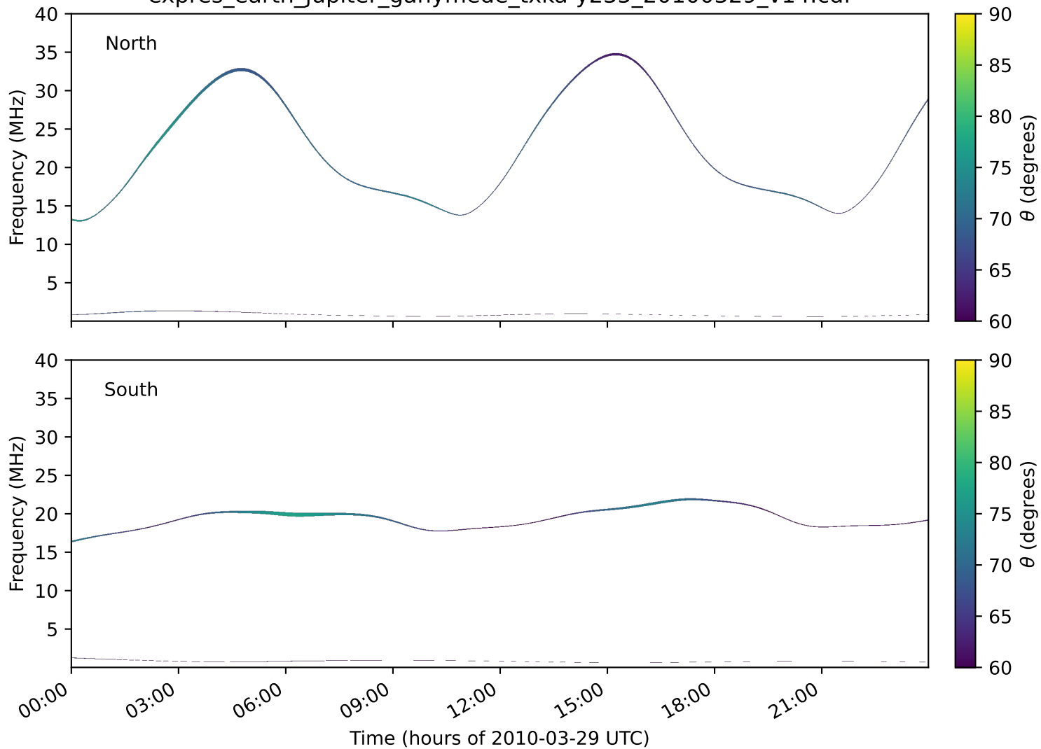
expres_earth_jupiter_ganymede_txka-y235_20100329_v14.cdf
