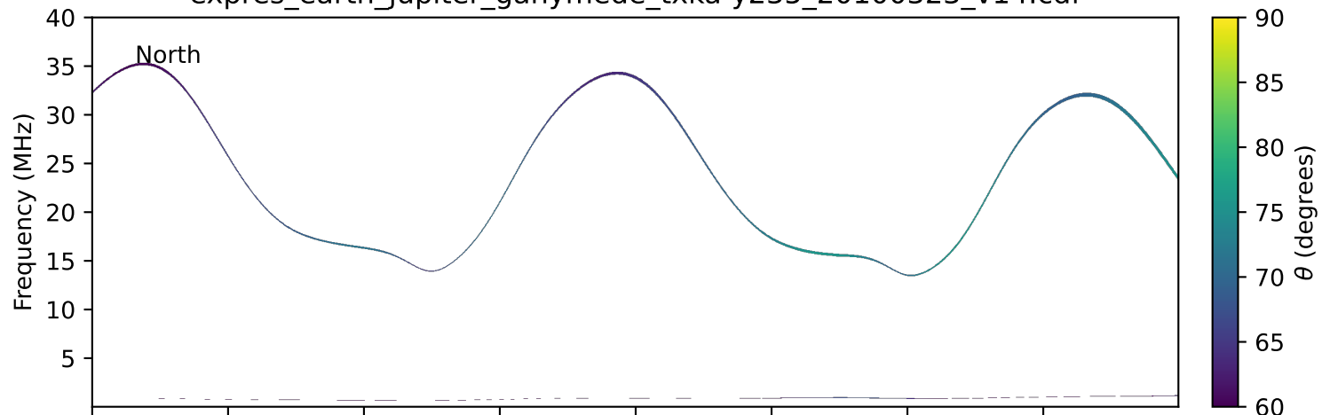
expres_earth_jupiter_ganymede_txka-y235_20100323_v14.cdf
