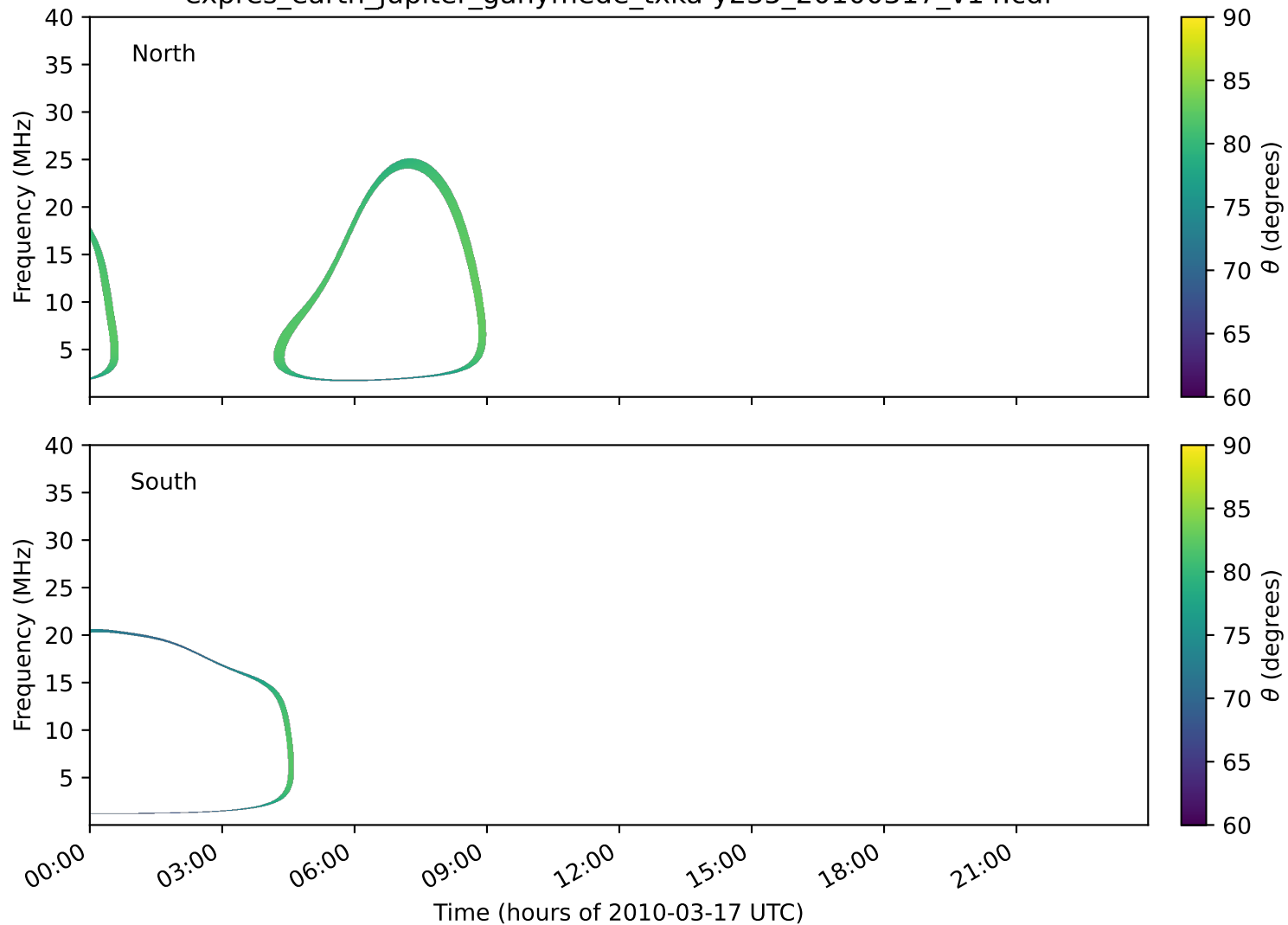
expres_earth_jupiter_ganymede_txka-y235_20100317_v14.cdf
