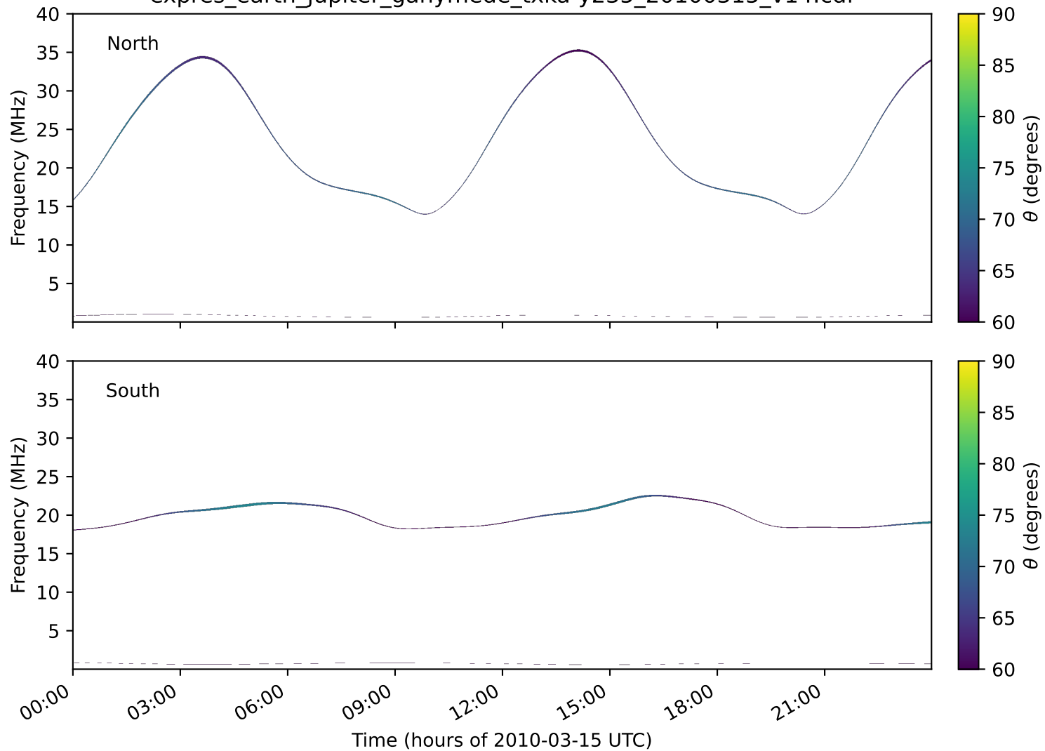
expres_earth_jupiter_ganymede_txka-y235_20100315_v14.cdf
