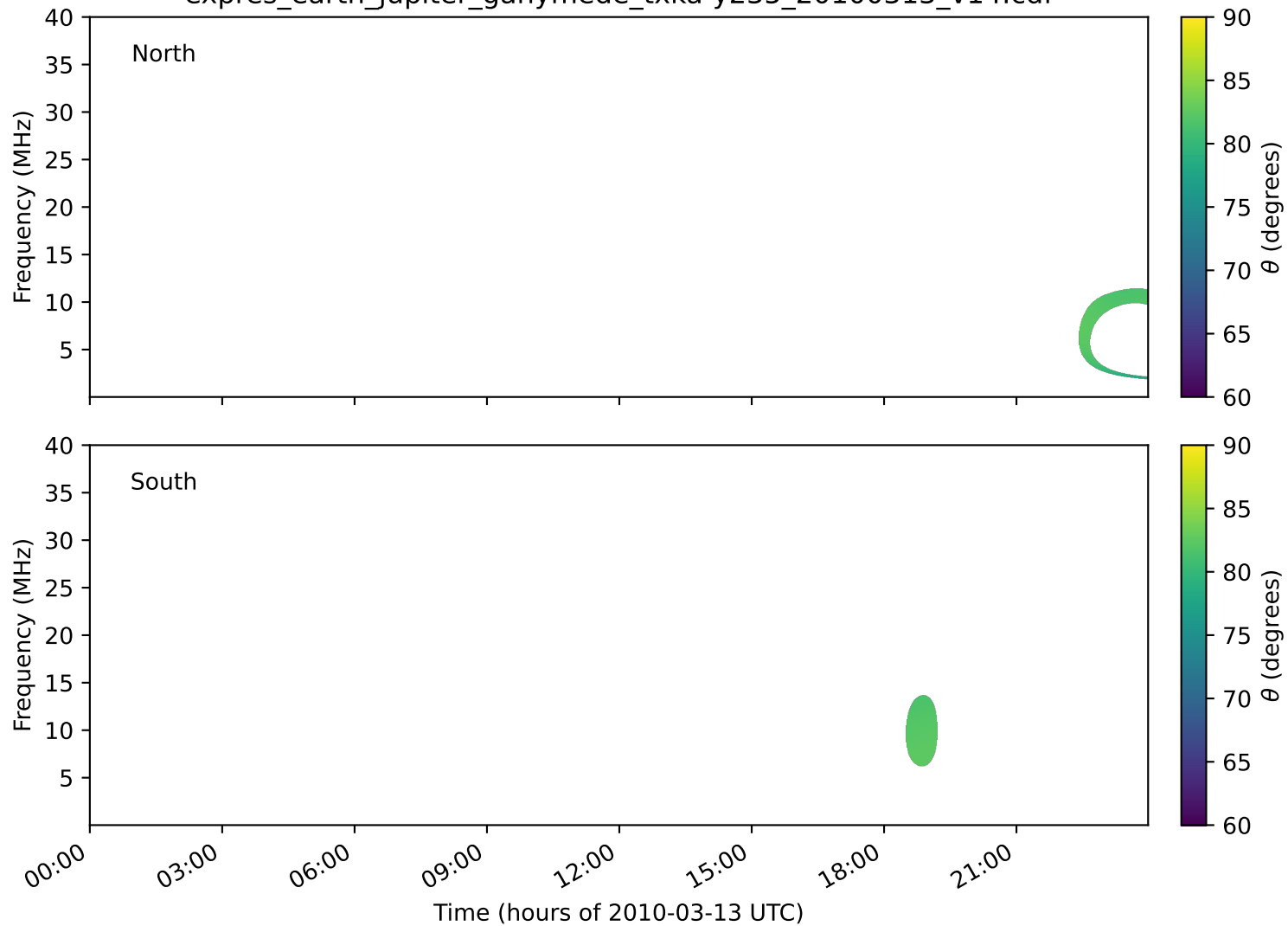
expres_earth_jupiter_ganymede_txka-y235_20100313_v14.cdf
